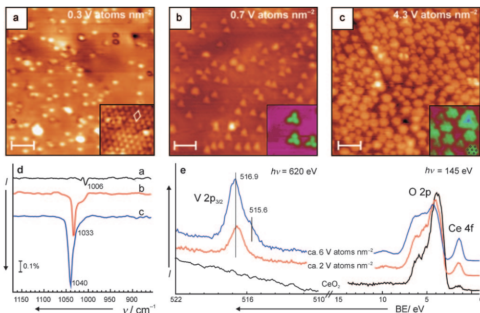
Figure 1. a–c) STM images of VO x /CeO 2 (111) for various vanadia loadings as indicated. Sample (a) was annealed to 300 K, while samples (b) and (c) were annealed to 700 K. The insets highlight the atomic structure of the vanadia deposits. The scale bars are 3 nm. Tunneling bias is 3 V; tunneling current is 0.02 nA (a), 0.01 nA (b), and 0.10 nA (c). d) IRA spectra of the vanadyl (V=O) stretching region for the corresponding STM images. e) PE spectra for two loadings of vanadia on CeO 2 (111) compared to a pristine CeO 2 (111) thin film.
